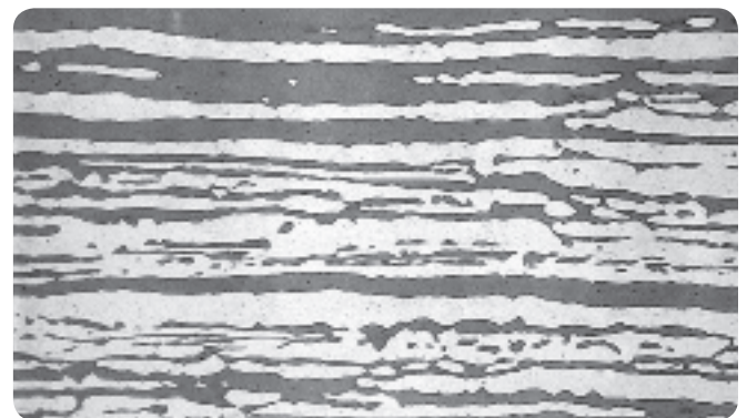
Typical Duplex Microstructure in 3/8-inch Plate, 500x.
