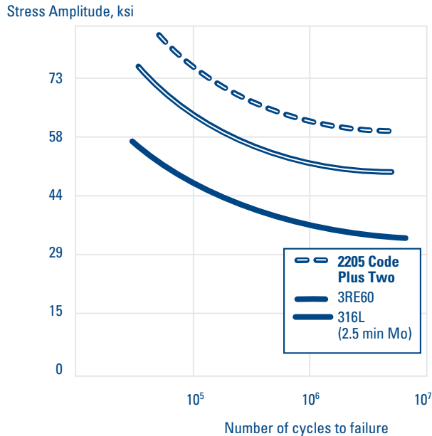
Smooth rotating bent beam at 1500 rpm (0.6-inch plate)
