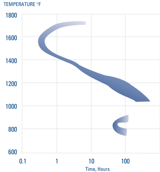
The curve corresponds to an ambient temperature Charpy V-notch impact toughness of 20 ft-lb
